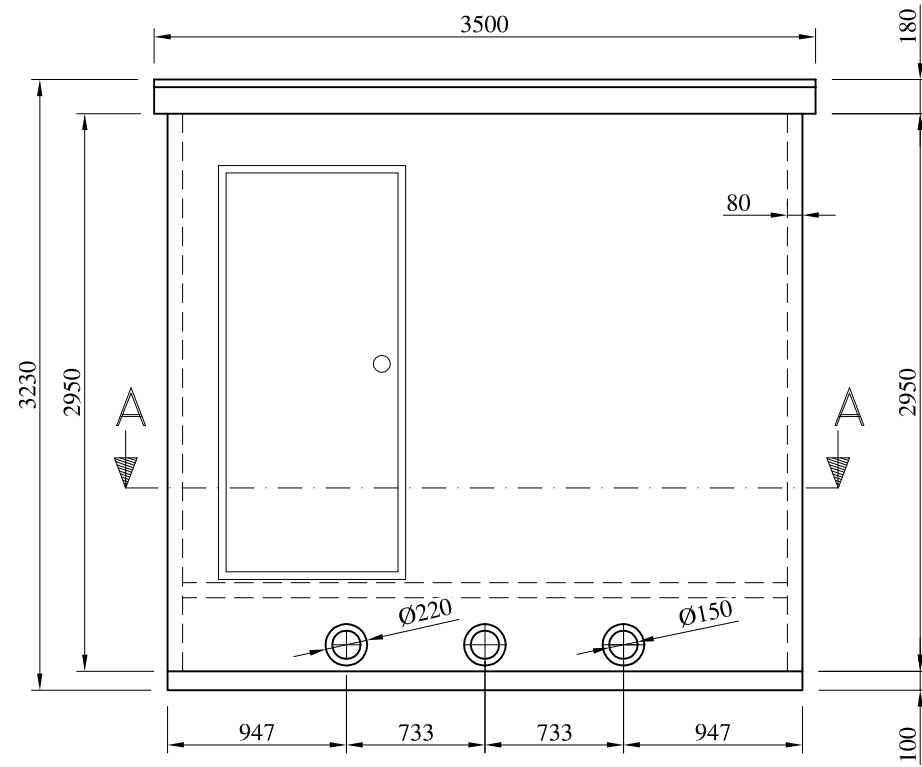
VISTA FRONTAL
