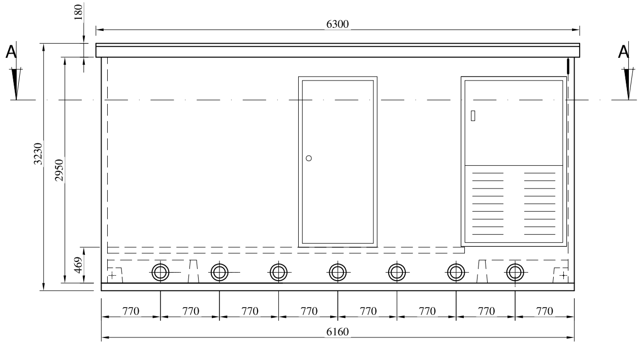
VISTA FRONTAL
